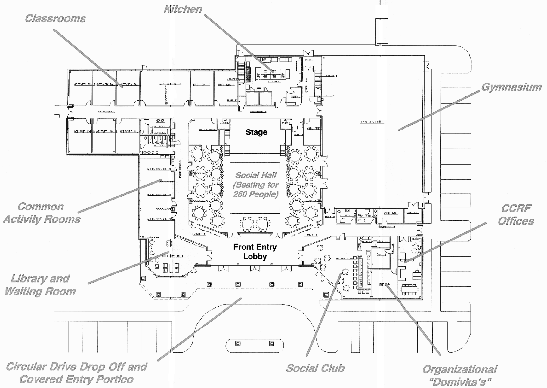
Cultural Center Floor Plan
